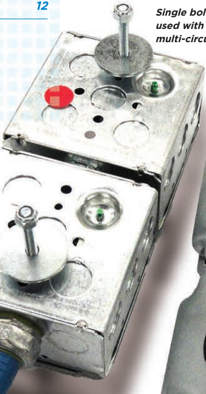
Uni-Strut Mounting Bolt (Single)
